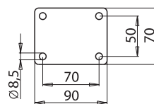
Priroba: za kolesa Ø100, Ø125 Top plate: for castors Ø100, Ø125
